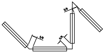
TYPICAL GLASS CORNERS DETAIL SCALE: 6"=1'-0"
