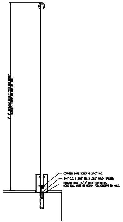
SECTION SCALE 3/4"=1'-0"
