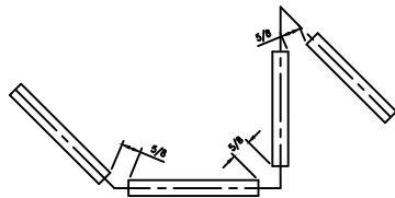
⊕ TYPICAL GLASS CORNERS DETAIL 6" = 1'-0"
