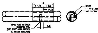
⊕ FACTORY CUT SPLICE 6" = 1'-0"
