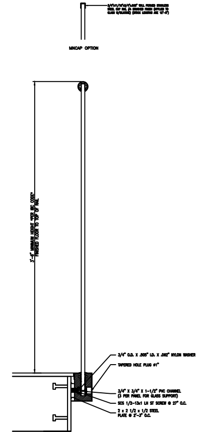
SECTION SCALE 3/4"=1'-0"
