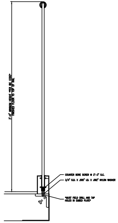
SECTION SCALE 3/4"=1'-0"
